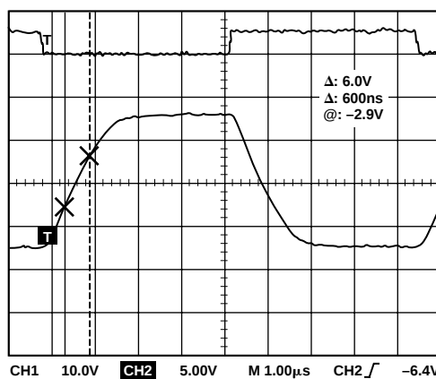
TPC 6. Transmitter Fully Loaded Slew Rate
