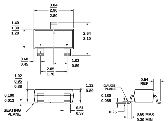
Figure 15. 3-Lead Small Outline Transistor Package [SOT-23] (RT-3) Dimensions shown in millimeters
