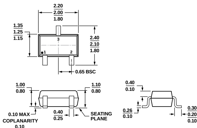
Figure 16. 3-Lead Thin Shrink Small Outline Transistor Package [SC70] (KS-3) Dimensions shown in millimeters
