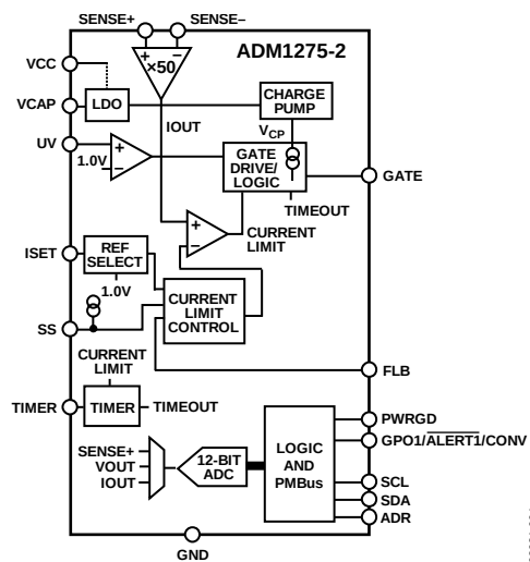
Figure 44. ADM1275-2 Functional Block Diagram
