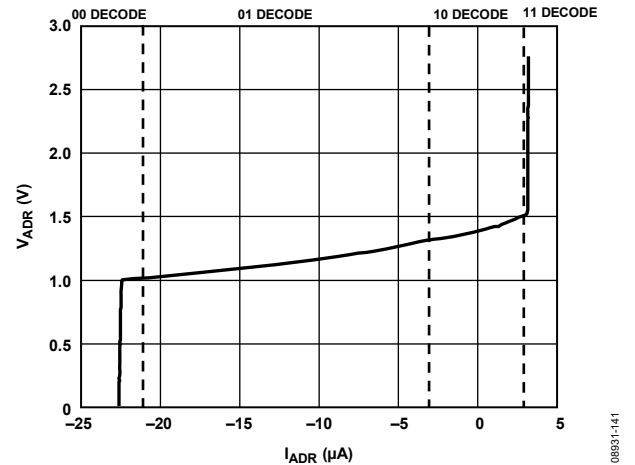
Figure 41. ADR Pin Voltage ( V_{ADR} ) vs. Current ( I_{ADR} )
