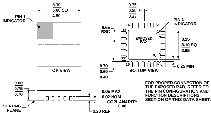
Figure 68. 20-Lead Lead Frame Chip Scale Package [LFCSP_WQ] 5 mm x 5 mm Body, Very Very Thin Quad (CP-20-9)
