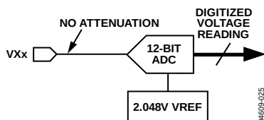
Figure 30. ADC Reading on VXx Pins
