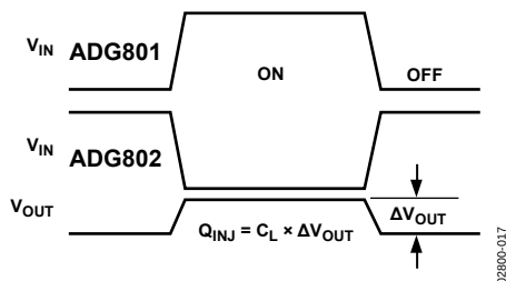
Figure 17. Charge Injection
