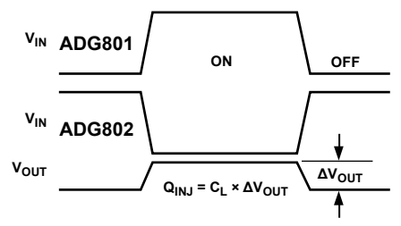
Figure 17. Charge Injection
