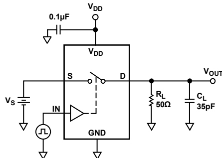
Figure 16. Switching Times
