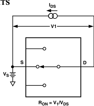
Test Circuit 1. R_{ON} Resistance
