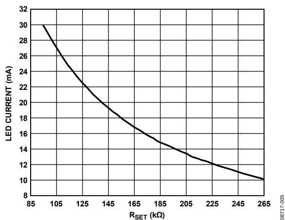
Figure 5. LED Current vs. R_{SET}
