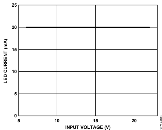
Figure 8. LED Current vs. Input Voltage ( I_{LED} = 20 mA)
