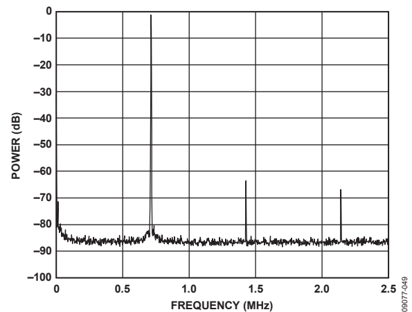
Figure 17. Power vs. Frequency, f_{CLK} = 5\text{ MHz} , f_{OUT} = 0.714\text{ MHz} = f_{CLK}/7 , Frequency Word = 0x2492492
