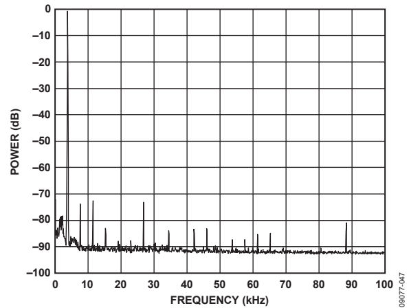
Figure 15. Power vs. Frequency, f_{CLK} = 16\text{ MHz} , f_{OUT} = 3.8\text{ kHz} , Frequency Word = 0x000FBA9
