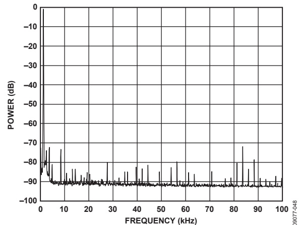
Figure 16. Power vs. Frequency, f_{CLK} = 5\text{ MHz} , f_{OUT} = 1.2\text{ kHz} , Frequency Word = 0x000FBA9
