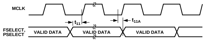
Figure 4. Control Timing
