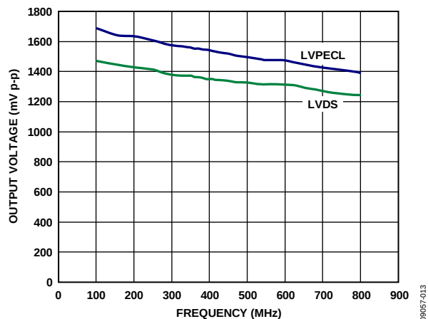
Figure 15. Peak-to-Peak Output Voltage vs. Frequency, LVPECL and LVDS (100 Ω Load)
