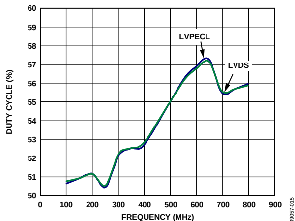
Figure 17. Duty Cycle vs. Output Frequency, LVPECL and LVDS (100 Ω Load)
