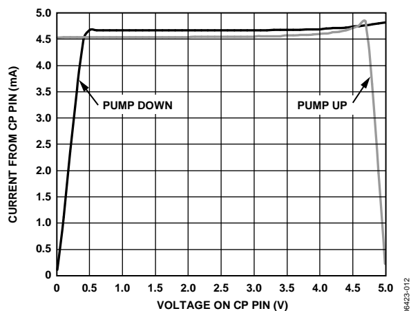
Figure 12. Charge Pump Characteristics at V_{CP} = 5.0\text{ V}
