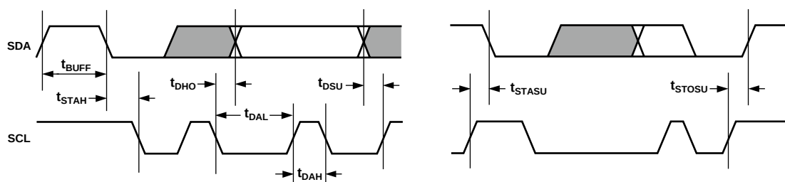
Figure 9. Serial Port Read/Write Timing
