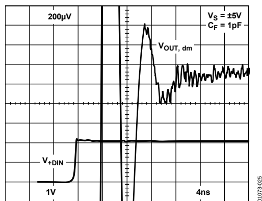
Figure 25. Settling Time
