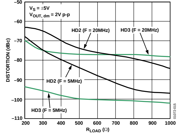
Figure 16. Harmonic Distortion vs. R_{L, dm}
