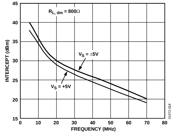
Figure 20. Third Order Intercept vs. Frequency
