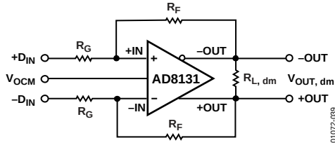
Figure 39. Circuit Definitions
