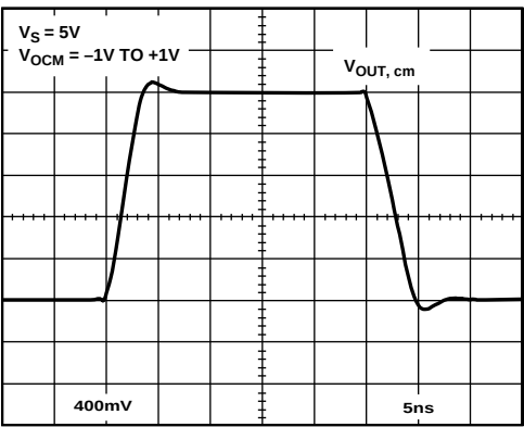
Figure 38. V_{OCM} Transient Response
