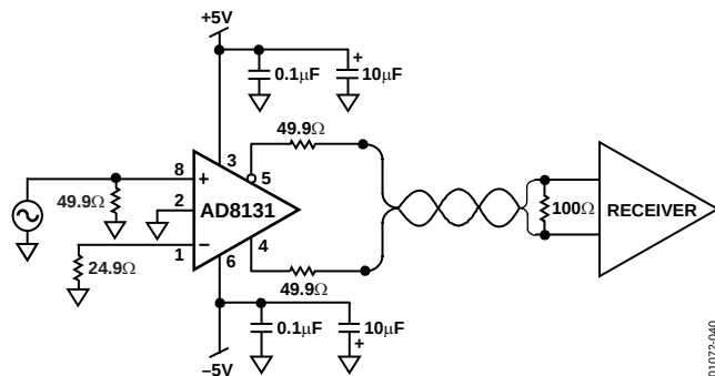
Figure 40. Single-Ended-to-Differential 100 \Omega Line Driver
