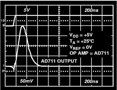
Figure 11. Digital-to-Analog Glitch Impulse
