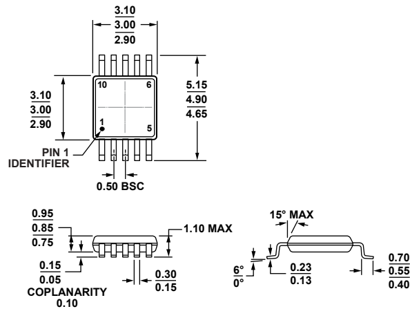
Figure 42. 10-Lead Mini Small Outline Package [MSOP] (RM-10) Dimensions shown in millimeters
