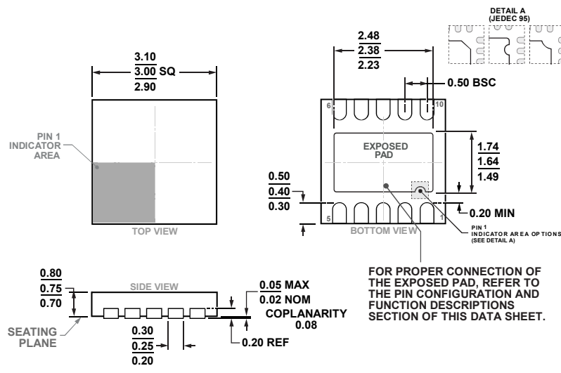
Figure 43. 10-Lead Lead Frame Chip Scale Package [LFCSP] 3 mm x 3 mm Body, Very Very Thin, Dual Lead (CP-10-9) Dimensions shown in millimeters
