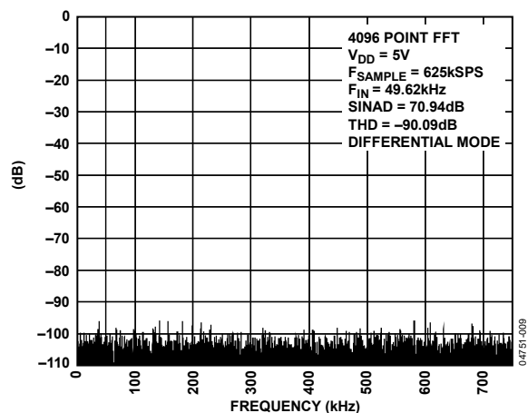
Figure 7. AD7938-6 FFT at V_{DD} = 5\text{V}
