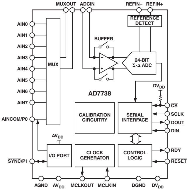
Figure 4. Block Diagram
