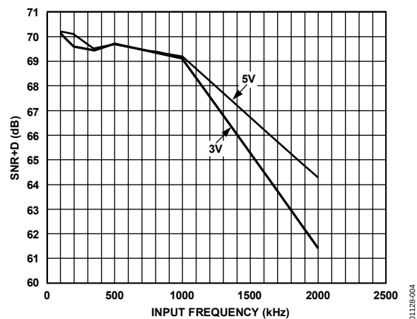
Figure 4. Typical SNR + D vs. Input Tone
