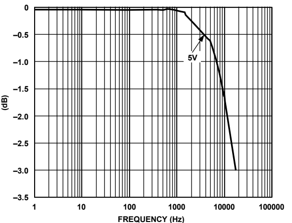
Figure 8. Typical Bandwidth
