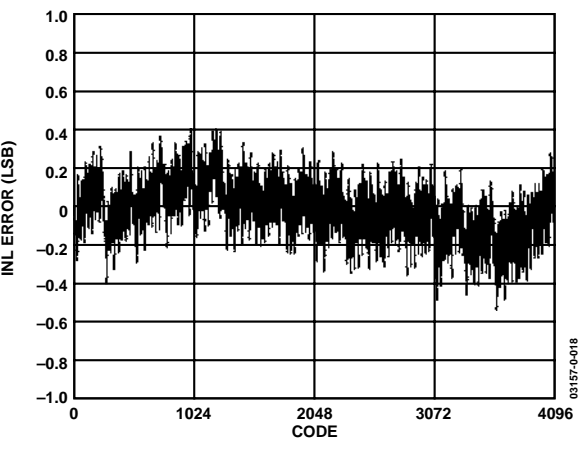
Figure 9. Typical INL for the AD7457 for V DD = 5 V
