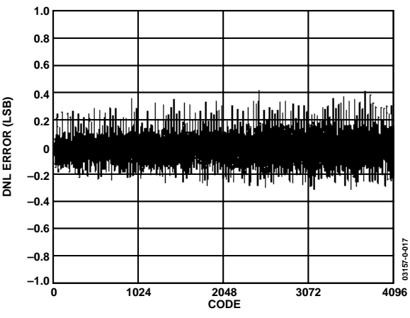
Figure 8. Typical DNL for the AD7457 for V DD = 5 V
