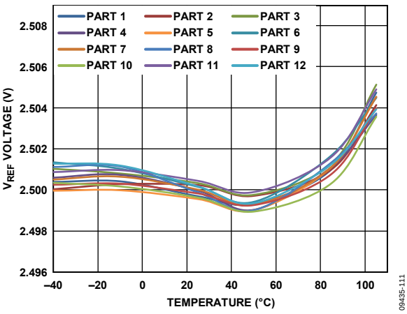
Figure 13. V REF vs. Temperature for Different Parts
