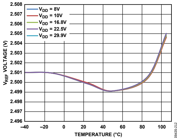
Figure 12. V REF vs. Temperature for Different Supply Voltages
