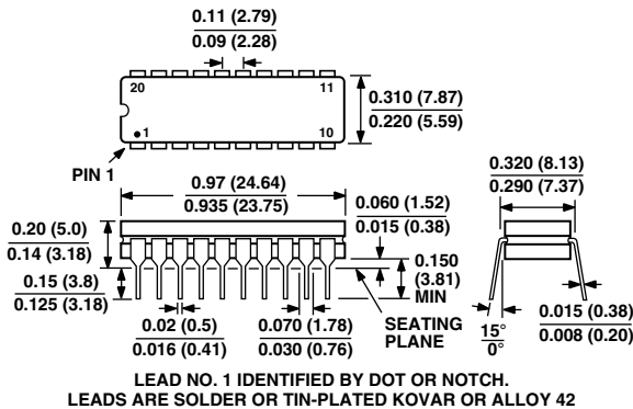
20-Lead Cerdip (Q-20)
