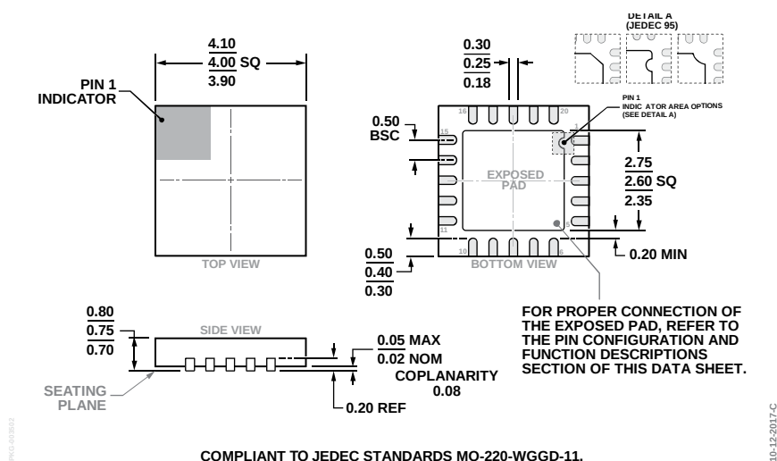
Figure 54. 20-Lead Lead Frame Chip Scale Package [LFCSP] 4 mm × 4 mm Body and 0.75 mm Package Height (CP-20-8)
