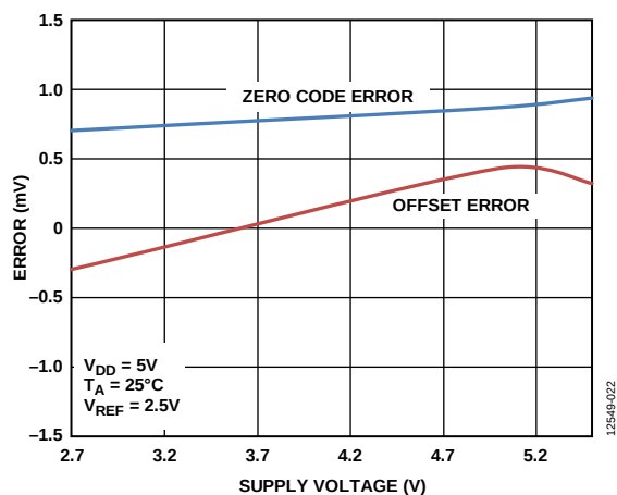
Figure 20. Zero Code Error and Offset Error vs. Supply Voltage
