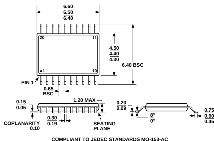
Figure 53. 20-Lead Thin Shrink Small Outline Package [TSSOP] (RU-20)
