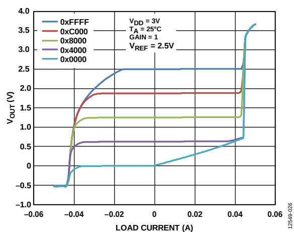
Figure 24. Source and Sink Capability at 3 V
