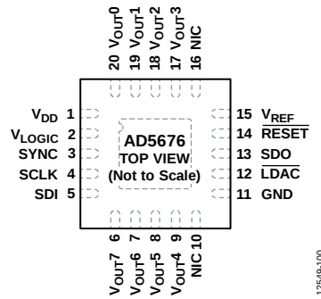
Figure 7. 20-Lead LFCSP Pin Configuration
