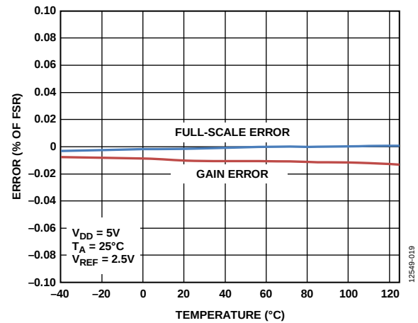
Figure 17. Gain Error and Full-Scale Error vs. Temperature
