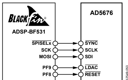
Figure 49. ADSP-BF531 Interface
