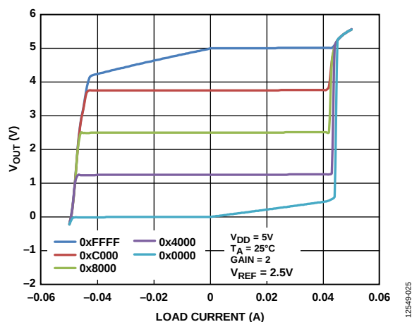
Figure 23. Source and Sink Capability at 5 V
