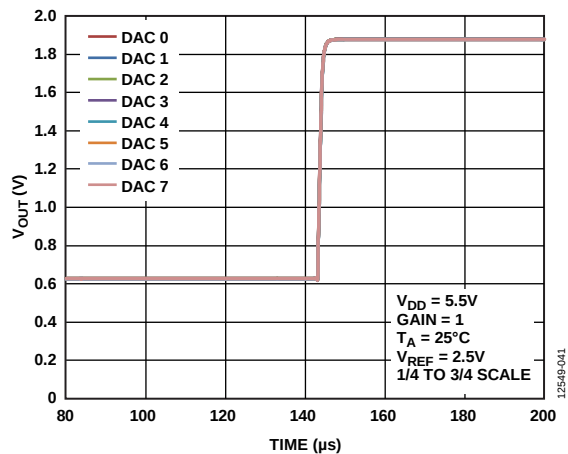
Figure 39. Settling Time, 5.5 V
