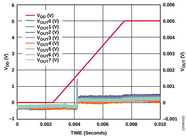
Figure 30. Power-On Reset to 0 V and Midscale
