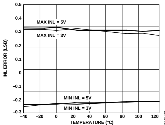
Figure 15. AD5622 INL Error vs. Temperature (3 V/5 V Supply)
