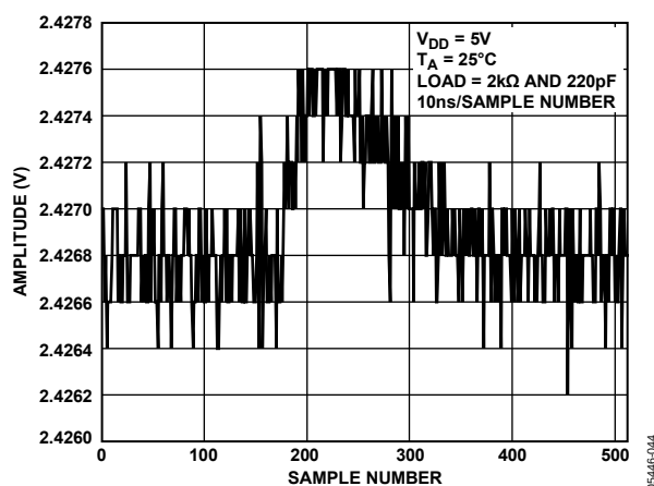
Figure 34. Digital Feedthrough
