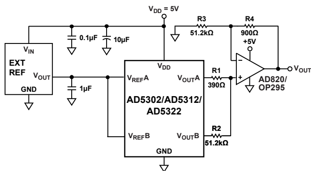
Figure 44. Coarse/Fine Adjustment
