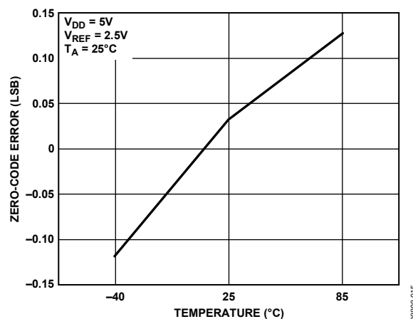
Figure 15. Zero-Code Error vs. Temperature
