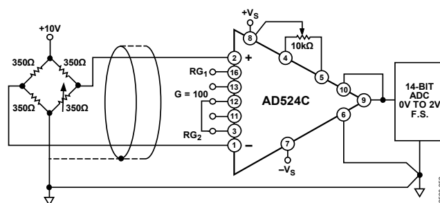
Figure 52. Typical Bridge Application
