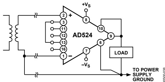
Figure 38. Indirect Ground Returns for Bias Currents—Transformer Coupled
