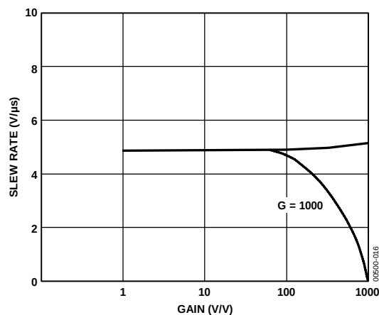
Figure 16. Slew Rate vs. Gain
