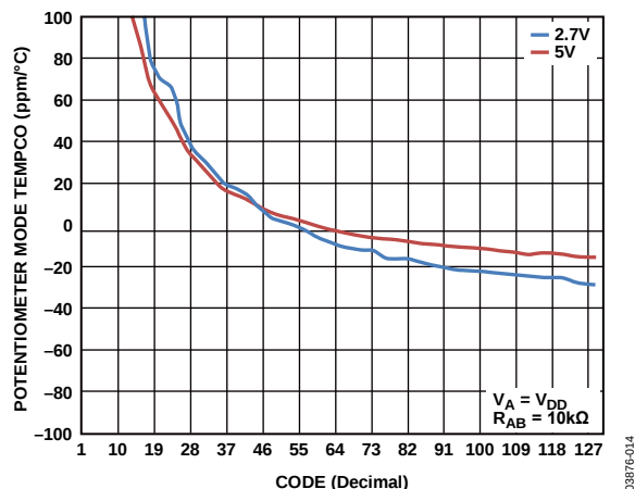
Figure 16. \Delta V_{WB}/\Delta T vs. Code
