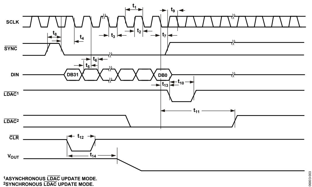
Figure 4. Serial Write Operation
