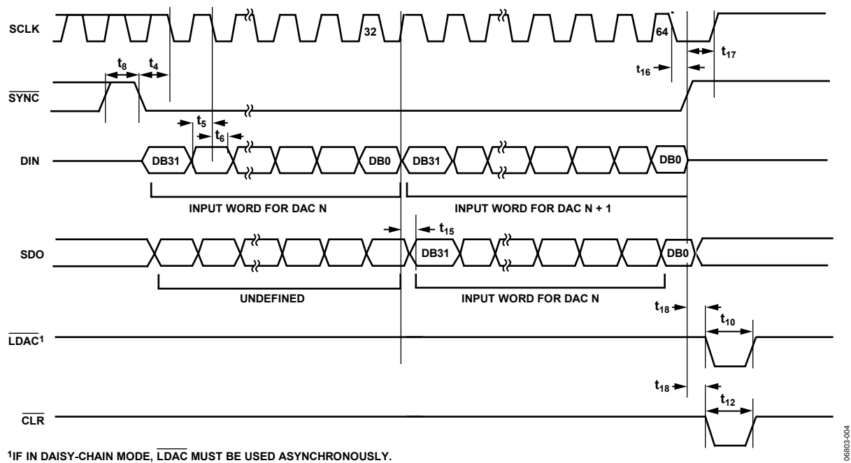
Figure 5. Daisy-Chain Timing Diagram
