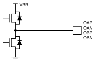
Figure 18i. Phase Outputs
