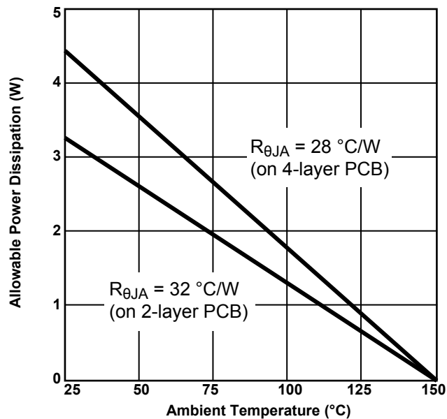
Figure 17: Allowable Power Dissipation, on Typical PCBs
