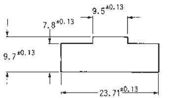
Panel Cutout (Applicable Board Thickness: 0.8–2.0 mm)
