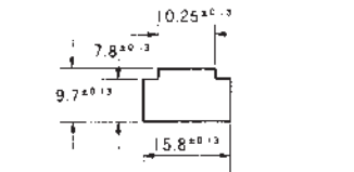
Panel Cutout (Applicable Board Thickness: 0.8–2.0 mm)
