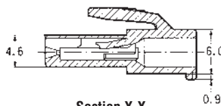
Section X-X
