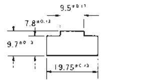
Panel Cutout (Applicable Board Thickness: 0.8–2.0 mm)
