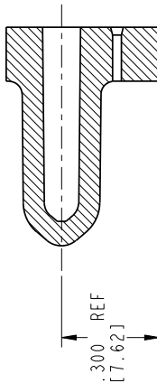
SECTION C-C SCALE 2:1
