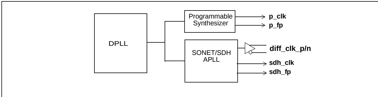
Figure 6 - Output Configuration
