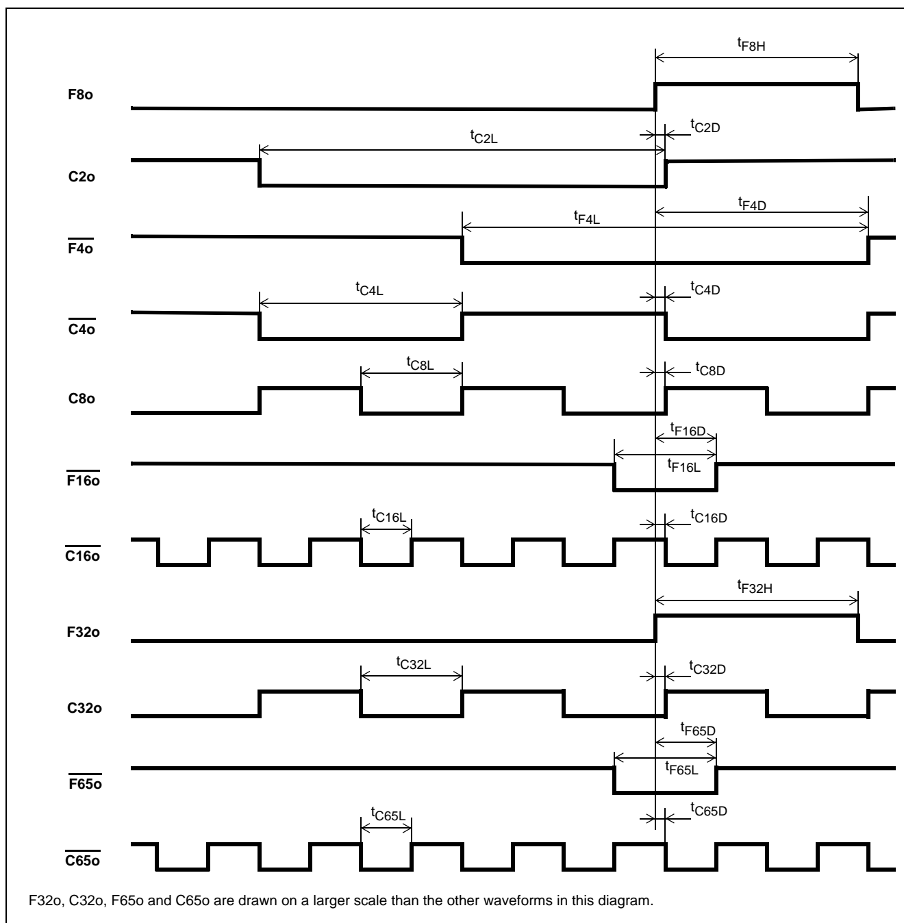
Figure 26 - E1 Output Timing Referenced to F8/F32o
