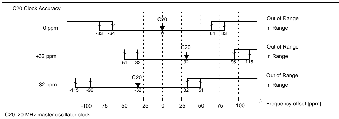
Figure 5 - DS1 Out-of-Range Thresholds for \text{OOR\_SEL}=0
