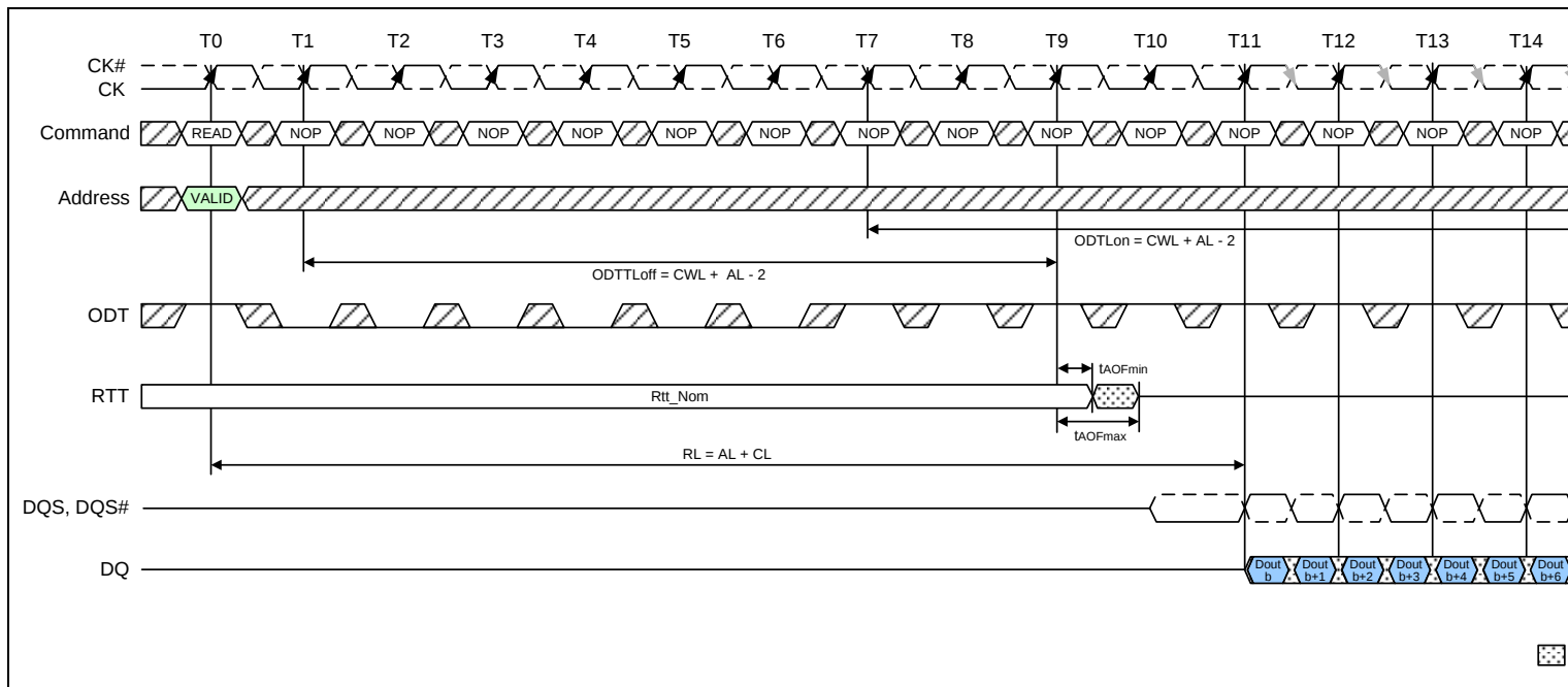
Figure 76 – ODT must be disabled externally during Reads by driving ODT low. (CL = 6; AL = CL - 1 = 5; RL = AL + CL = 11; CWL = 5; ODTLon = CWL + AL - 2 = 8; ODTLoft = CWL + AL - 2 = 8)
