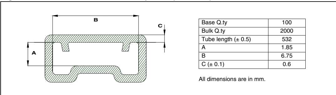
Figure 36. PowerSSO-12™ tube shipment (no suffix)
