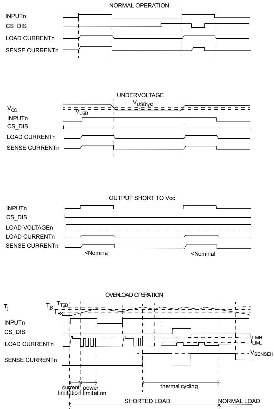
Figure 6. Waveforms
