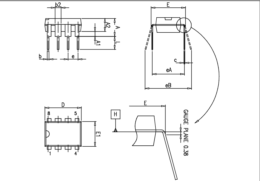
Figure 16. Package dimensions
