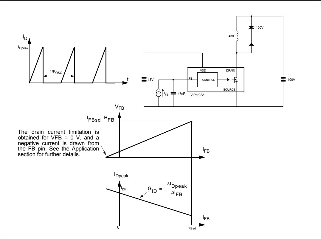
Figure 12. Peak drain current vs feedback current
