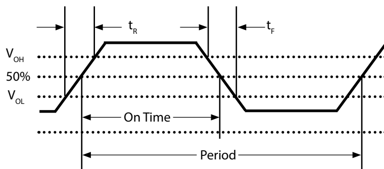
Fig 2: Waveform
