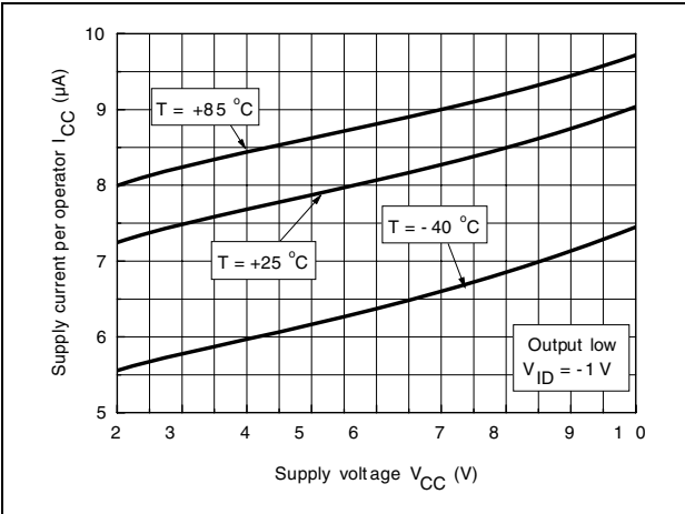
Figure 9. Supply current ( I_{CC} ) vs. supply voltage ( V_{CC} ) ( V_{ID} = -1\text{ V} )
