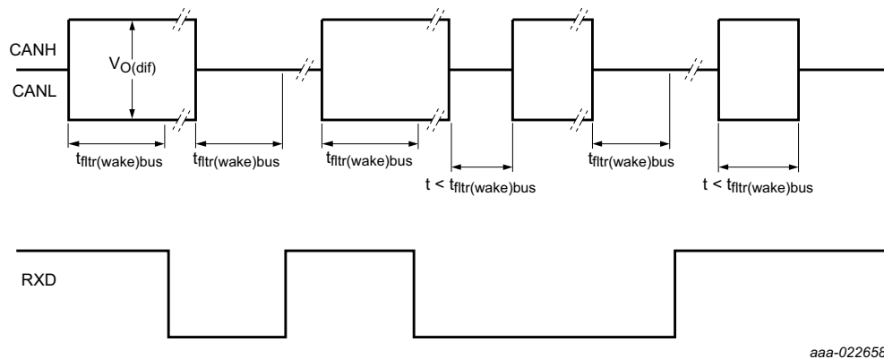
Fig 3. Wake-up timing
