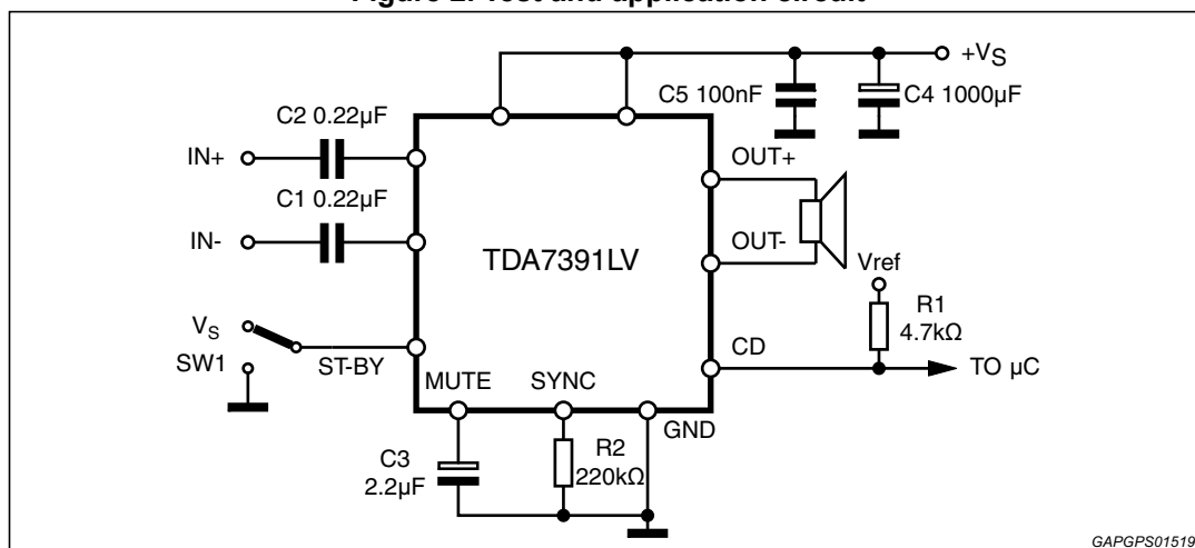
Figure 2. Test and application circuit
