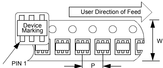
Component Taping Orientation for 5-Pin SOT-23A (EIAJ SC-74A) Devices
