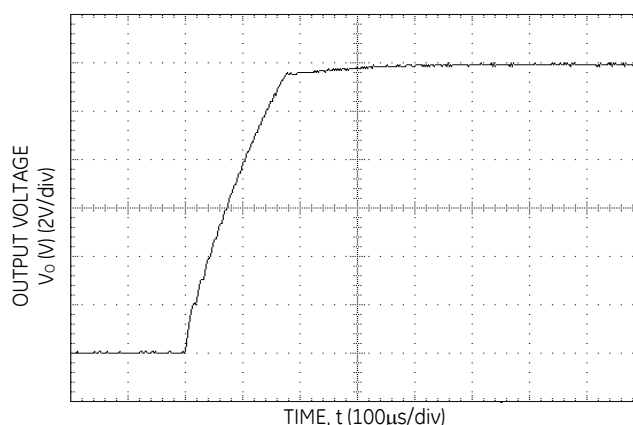
Figure 12. Typical Start-Up Output Voltage Rise Characteristic.
