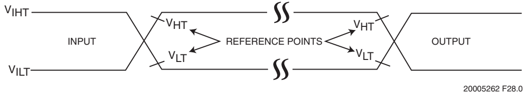
FIGURE 8-5: AC INPUT/OUTPUT REFERENCE WAVEFORMS
