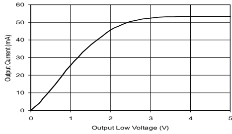
Output Current vs Receiver Output Low Voltage
