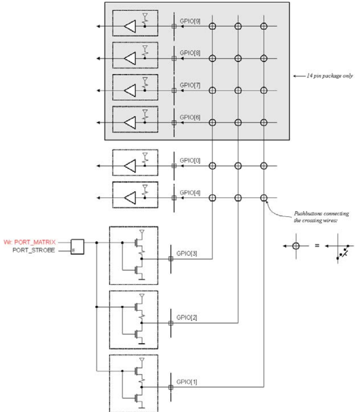
Figure 30.4. Push Button Organization in Matrix Mode
