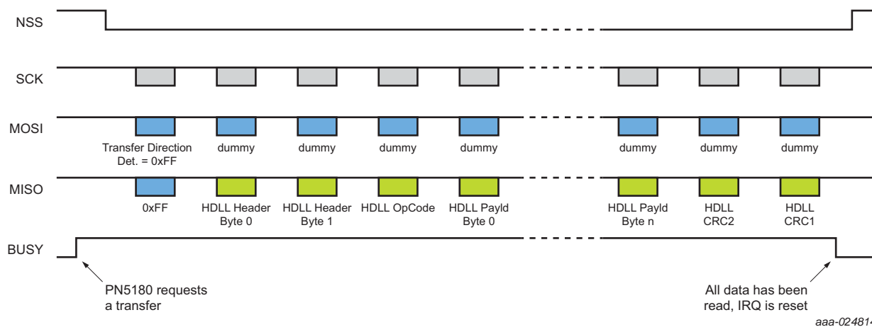
Fig 43. Secure Firmware Download: SPI Read
