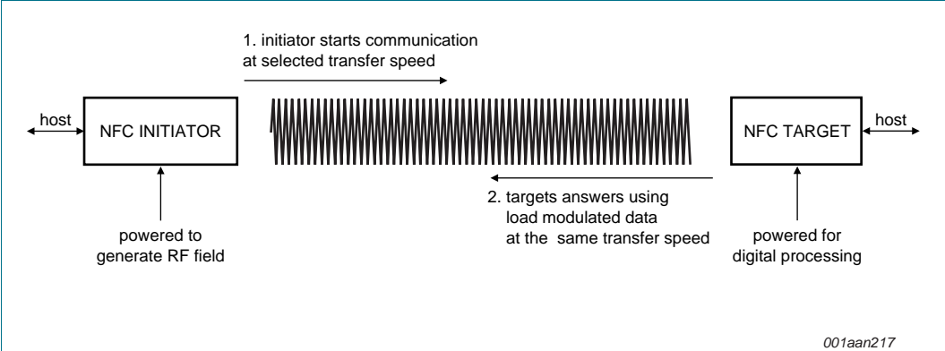
Fig 27. Passive communication mode
