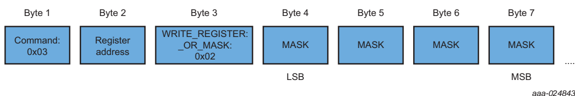
Fig 13. WRITE_REGISTER_OR_MASK
