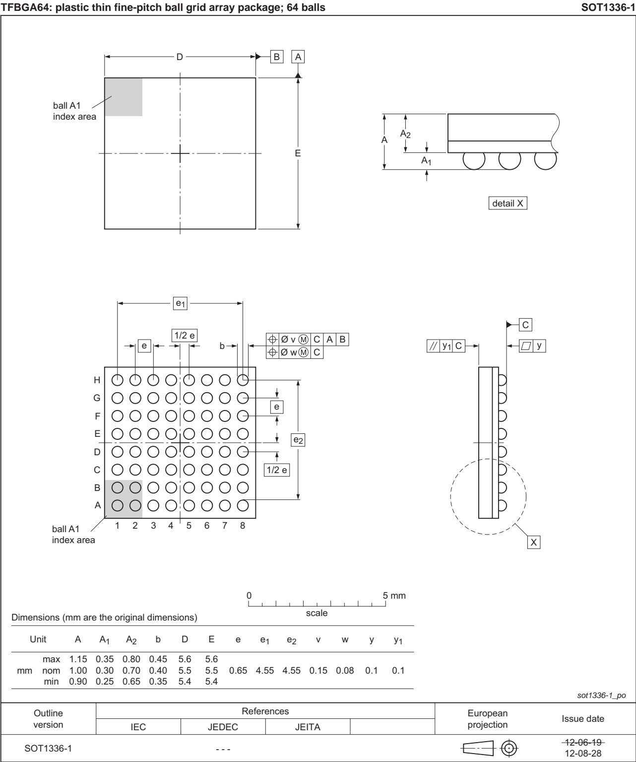
Fig 53. Package outline package version (TFBGA64)
