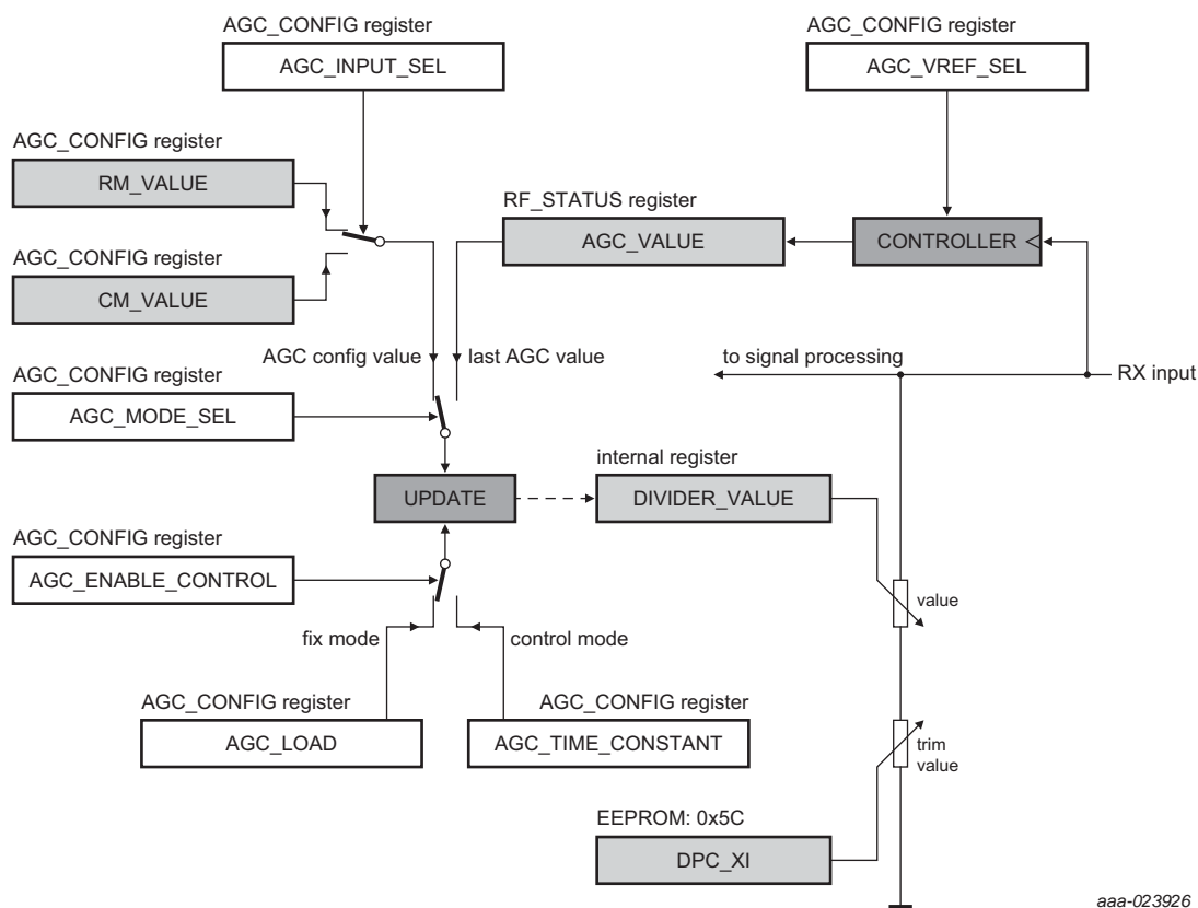
Fig 35. DPC, AGC and AWC configuration
