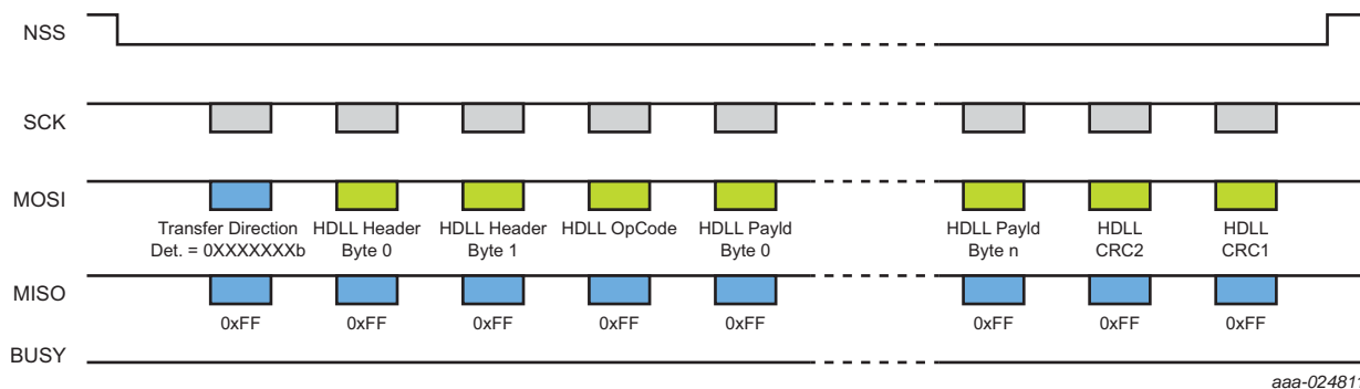
Fig 42. Secure Firmware Download: SPI Write
