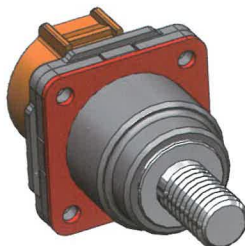
终端形式：螺栓 Termination Type: Thread Bolt
